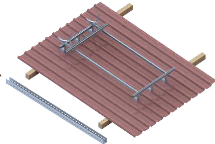
TRAPEZ ÇATI APARATI / TRAPEZE ROOF COMPONENT
