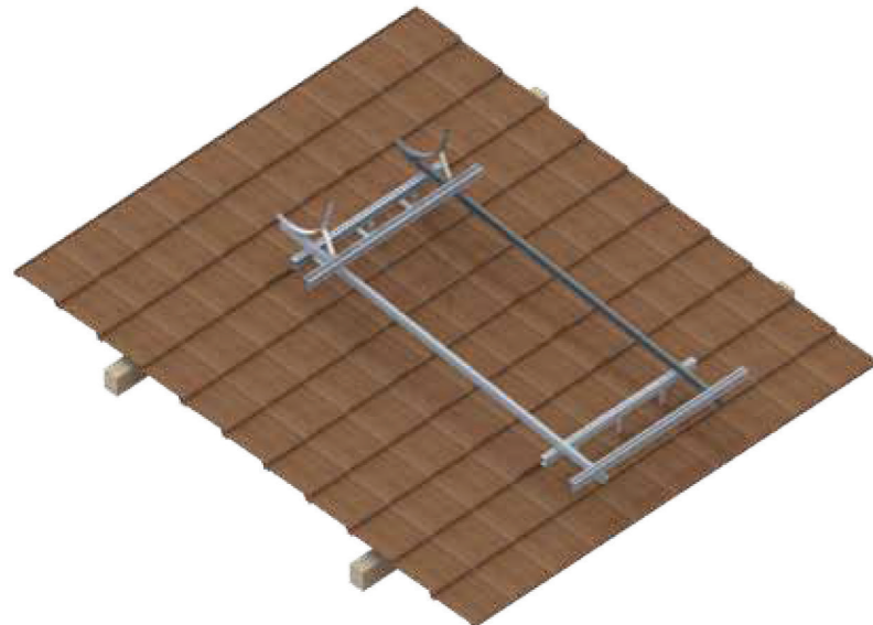
KİREMİT ÇATI APARATI / TILE ROOF COMPONENT
